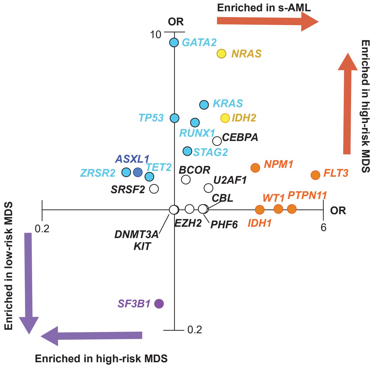
Figure 1. Enrichment of mutations in s-AML and high risk MDS versus high-risk and low-risk MDS respectively. Enrichment of mutations expressed as odds ratio (OR) of mutation rates in s-AML vs high risk MDS (x-axis) and in high risk MDS vs low risk MDS (y-axis). Non-significant OR are represented by black circles. Adapted from 26 .
